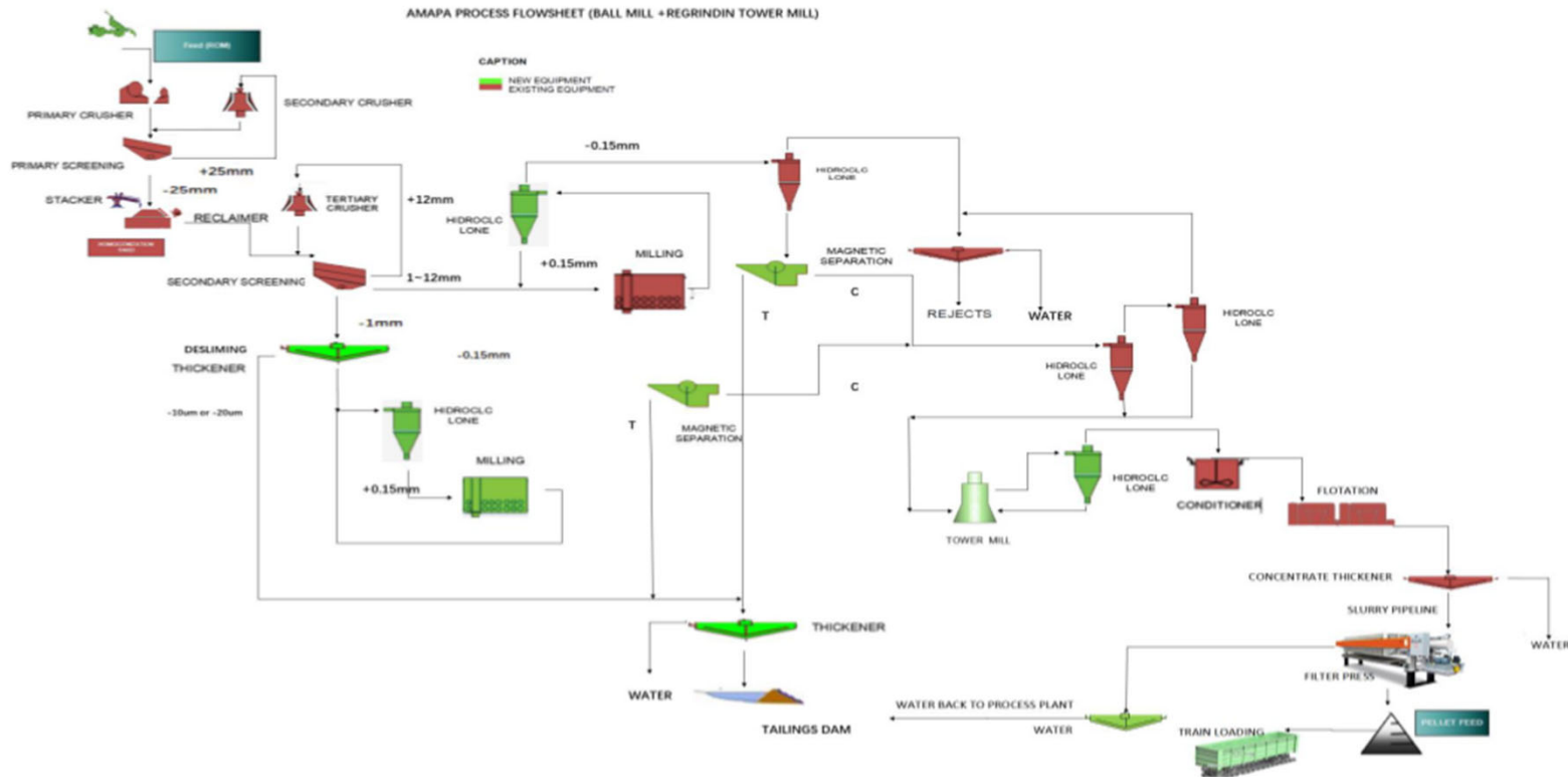
Figure 3-2 PSEI Proposed Flowsheet
